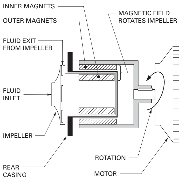
FIGURE 2: PUMP MAGNETIC DRIVE
